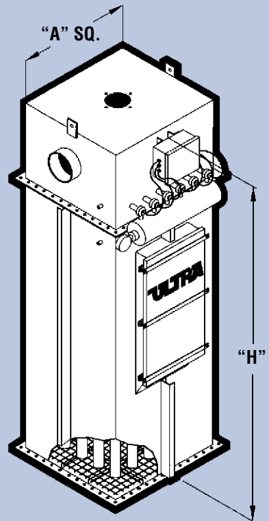
ARRANGEMENT IIG (GRID PLATFORM STANDARD)
